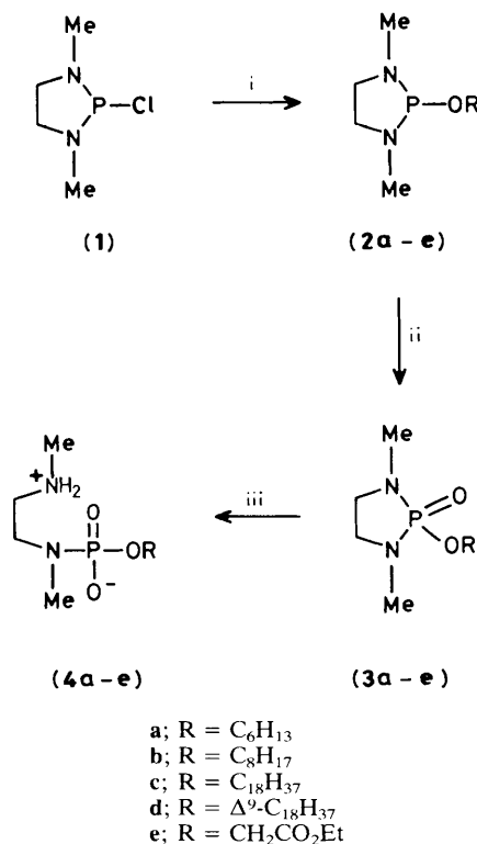
Scheme 1. Reagents: i, ROH-Et 3 N, CH 2 Cl 2 , -60°C; ii, N 2 O 4 , CH 2 Cl 2 , -60°C; iii, aq. HCl, THF.
